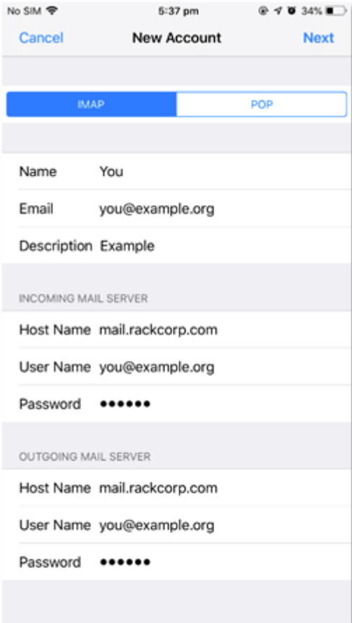
Figure 48 fill in the email account and server details as illustrated
