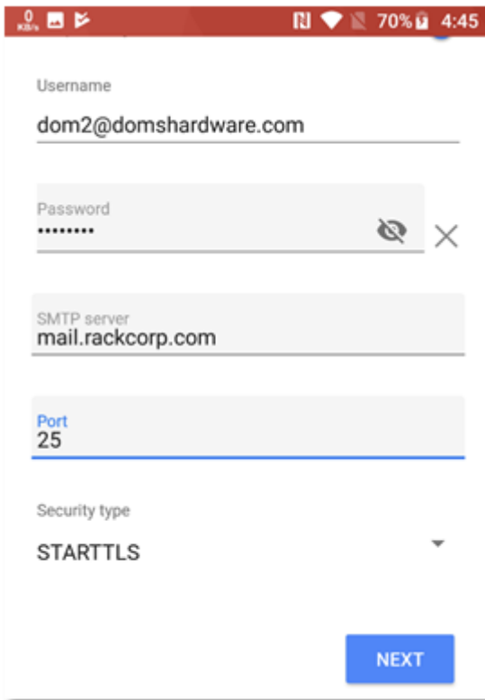
Figure 32 change the OUTGOING mail server to mail.rackcorp.com . Change the port to 25 and security to STARTTLS
