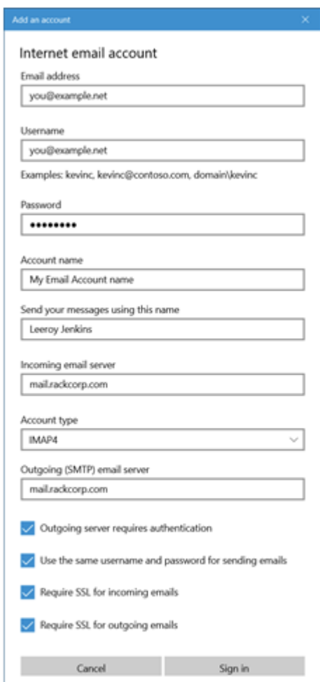
Figure 16 Windows 10 mail manual setup for RackCorp POP/IMAP email - fill in the details as illustrated, choose IMAP or POP
